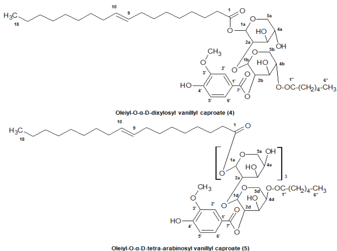
Fig 2: Structural formulae of the compounds 4 and 5 isolated from the leaves of Nyctanthes arbor-tristis
