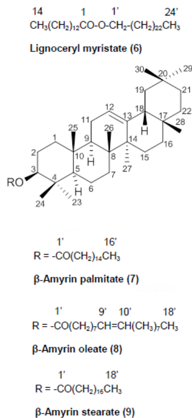
Fig 3: Structural formulae of the compounds 6 - 9 isolated from the roots of Verbesina encelioides
