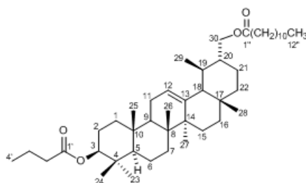
30-Lauryloxy- \alpha -amyrin-3-butyrate (2)
